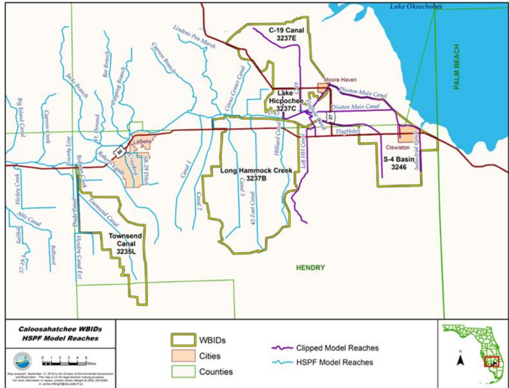
Figure 4.1. Model reaches in the tributary WBIDs for the full Caloosahatchee HSPF Model and the clipped Caloosahatchee HSPF Model
