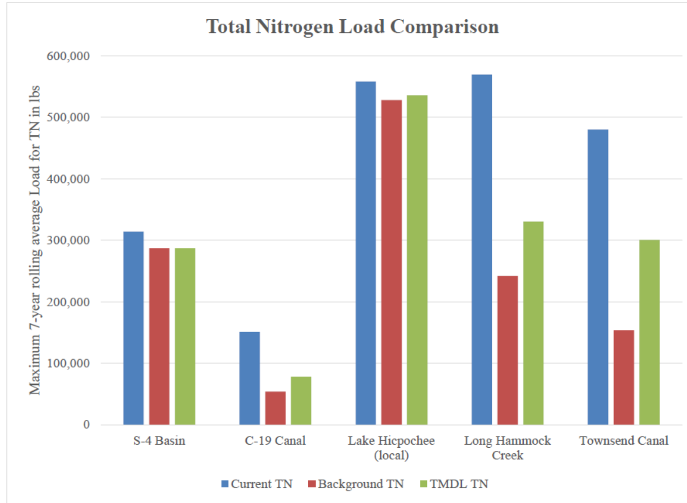
Figure 4.4. Simulated TN loads for each WBID from the current, background, and TMDL model runs. Note that for comparability the loads shown for Lake Hicpochee are for the local watershed without the upstream contribution.
