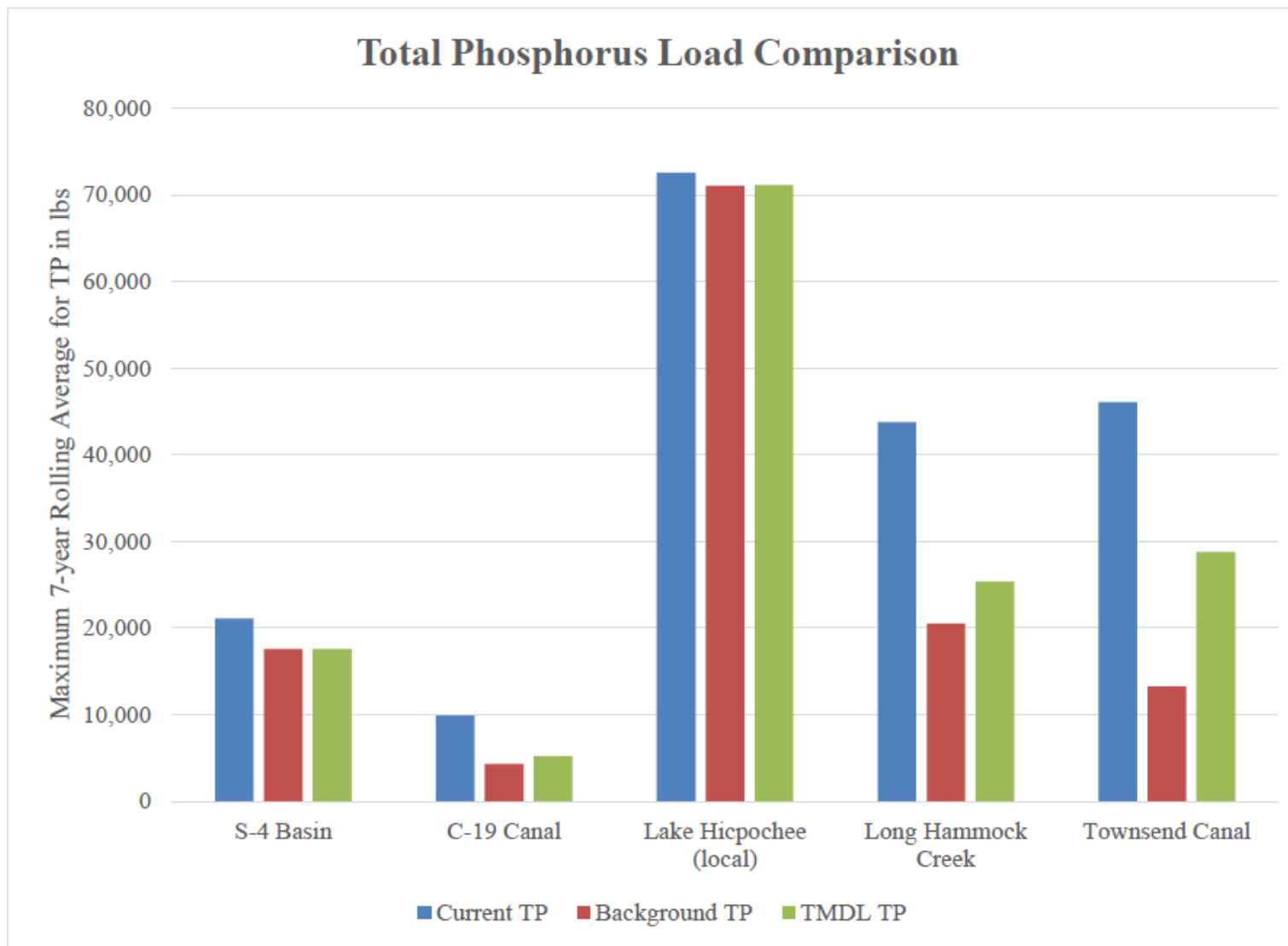
Figure 4.5. Simulated TP loads for each WBID from the current, background, and TMDL model runs. Note that for comparability, the loads shown for Lake Hicpochee are for the local watershed without the upstream contribution.
