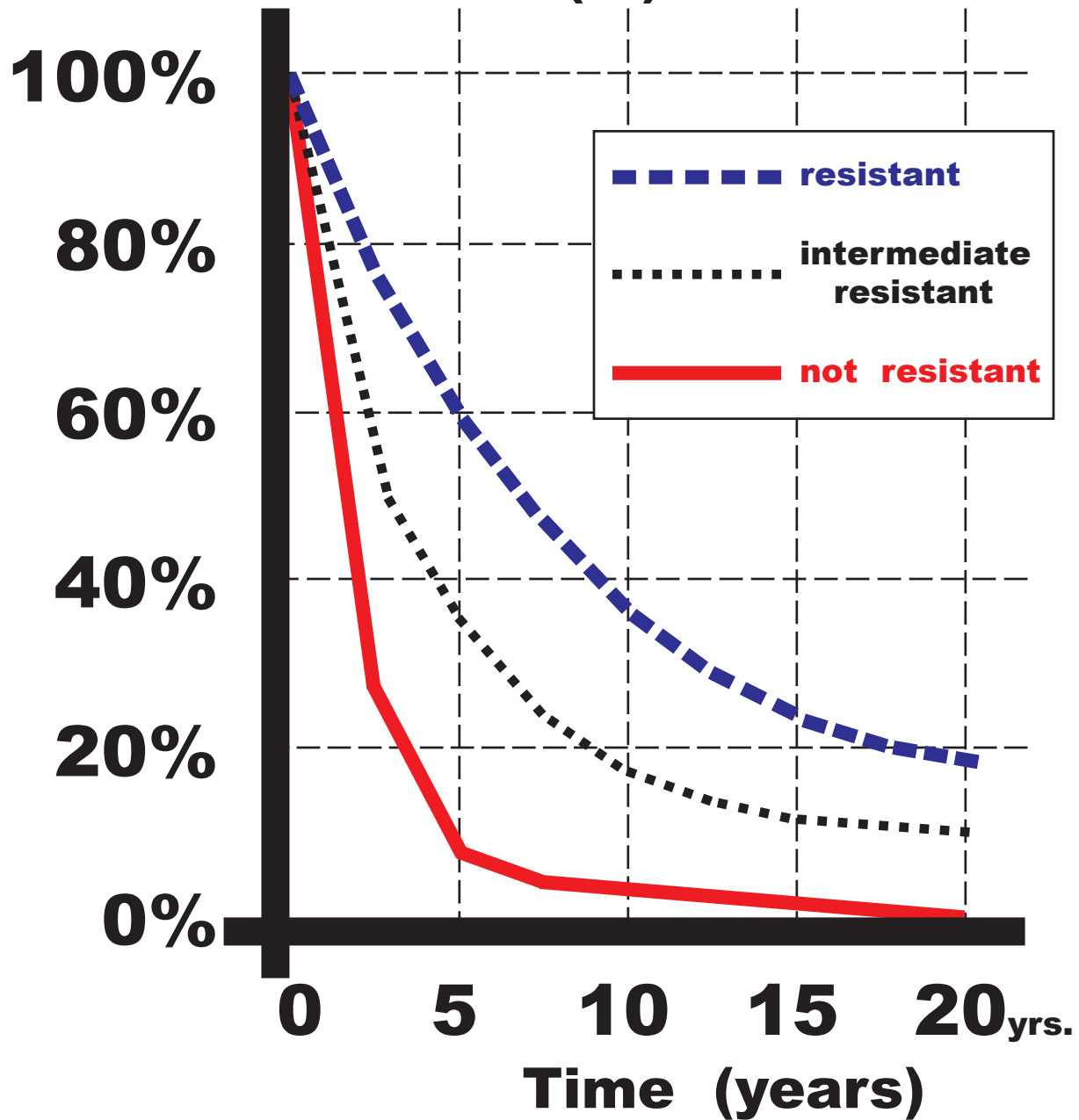
Figure 14: Graphical description of how rapidly wood decays from various tree species with different levels of heartwood resistance to decay. (after Sidle, 1991)
